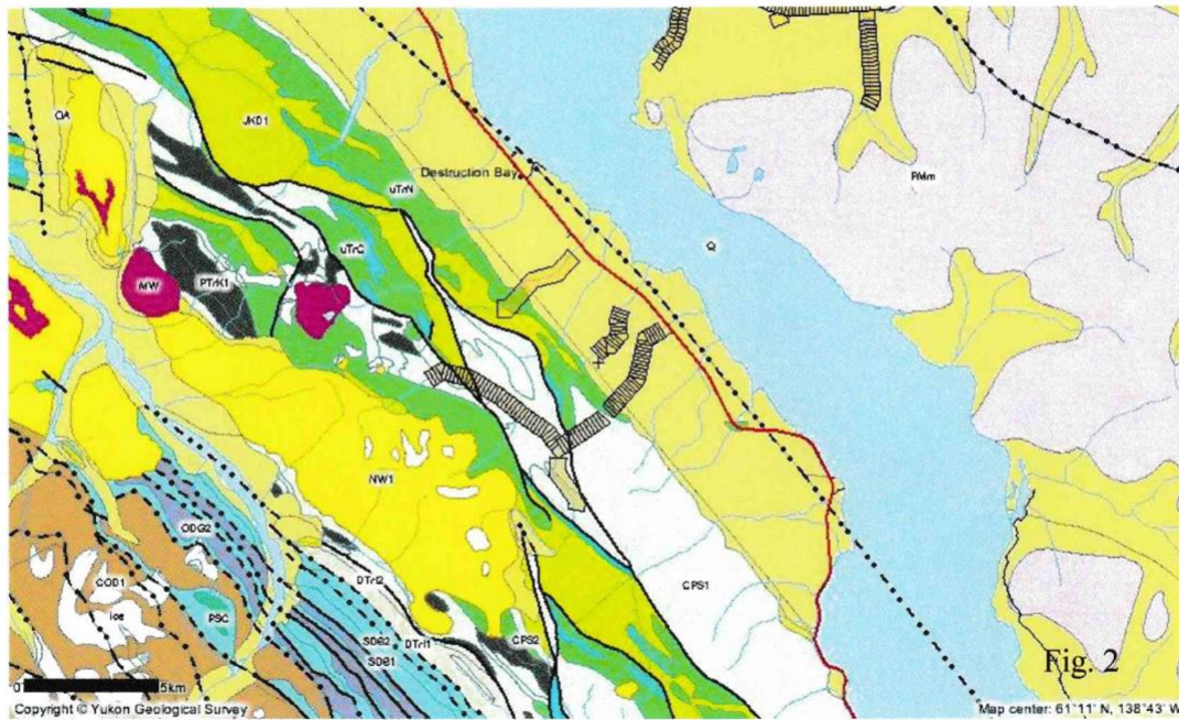
Fig. 2: Regional Geology
